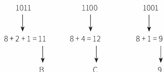
Figure 1.09 Converting a binary number into hexadecimal
