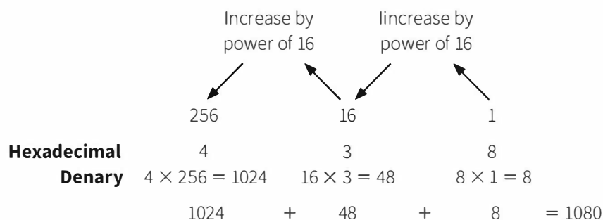
Figure 1.08 Hexadecimal notation for denary number 1080
