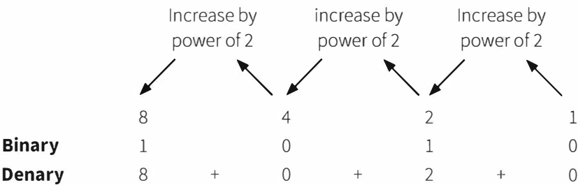
Figure 1.02 Converting a binary number into a denary number
