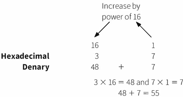
Figure 1.07 Converting a denary number into hexadecimal
