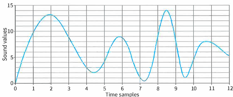
Figure 1.14 Sound wave
