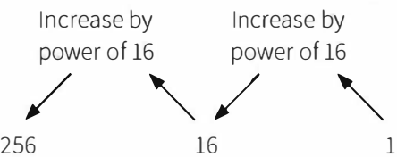
Figure 1.06 Hexadecimal base-16 number system
